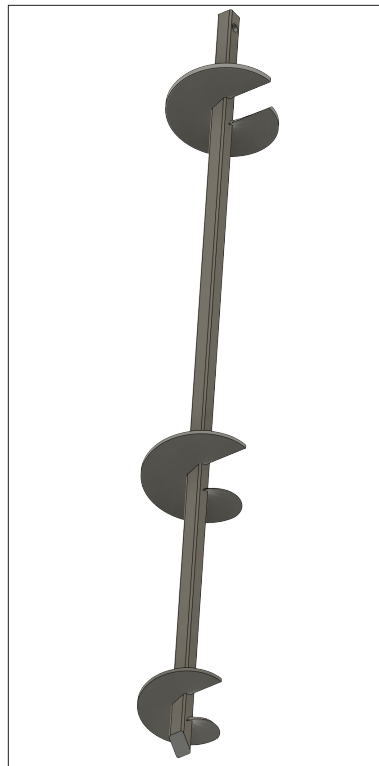
The lower two flights on the HGA have “C” shape chisel flight finish. Top flight has standard straight flight finish.
